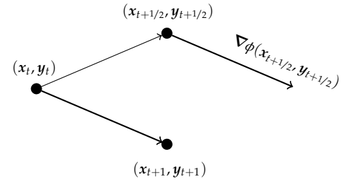
Figure 14.1. Illustration of a single step of the extragradient method.
