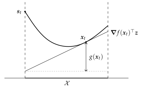
Figure 7.1. Illustration of a Frank-Wolfe step. As can be seen, \mathbf{s}_t is the minimizer of \nabla f(\mathbf{x}_t)^\top \mathbf{z} and is on the edge of \mathcal{X} . Furthermore, it shows the duality gap g(\mathbf{x}_t) .
