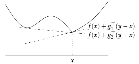
Figure 10.1. \mathbf{g} is a subgradient of f at \mathbf{x} if the whole graph is above \mathbf{x} 's supporting hyperplane, parametrized by \mathbf{g} .
