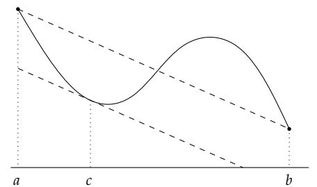
Figure 2.1. Illustration of the mean value theorem.
