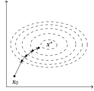
Figure 3.1. Gradient descent updates.
