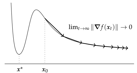
Figure 6.2. Gradient may get stuck in a flat region (saddle point) in nonconvex functions.
