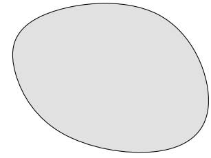
Figure 2.2. Example of a convex set in \mathbb{R}^2 .
