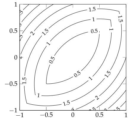
Figure 5.1. Level set plot of f(\mathbf{x}) = \|\mathbf{x}\|^2 + |x_1 - x_2| . The global minimum is [0, 0] , but greedy coordinate descent cannot escape any point [x, x] , s.t. |x| \leq 1/2 .
