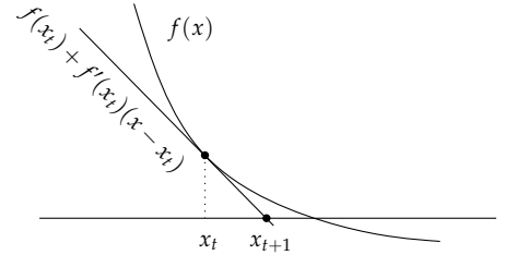
Figure 8.1. A step of the Newton-Raphson method.
