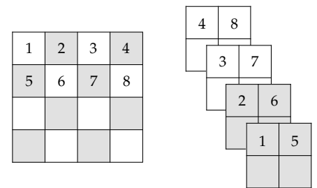
Figure 8.2. Masking used by RealNVP [Dinh et al., 2016].
