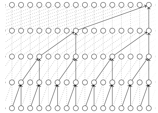
Figure 7.4. Stacked dilated convolutional layers in WaveNet .
