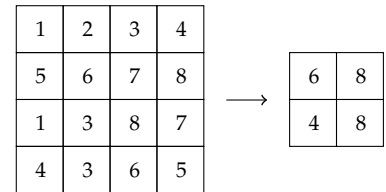
Figure 2.4. Toy example of max pooling.
