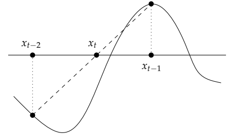
Figure 12.2. Illustration of the secant method.
