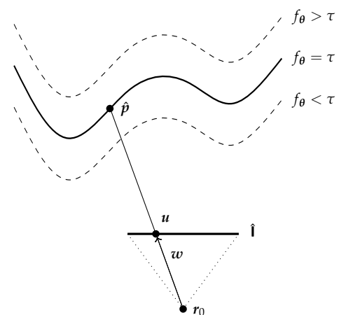
Figure 12.1. To render an object from the occupancy network f_\theta and texture field t_\theta , we cast a ray with direction w through a pixel u and determine the intersection point \hat{p} with the isosurface f_\theta(\hat{p}) = \tau . Afterward, we evaluate the texture field t_\theta(\hat{p}) to obtain the color prediction \hat{\mathbf{I}}_u .
