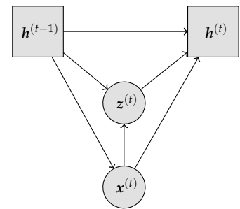
Figure 7.5. Computational graph of VRNN for inference.
