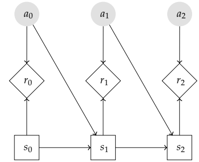
Figure 11.1. Diagram of an MDP.
