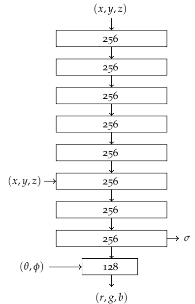
Figure 12.3. NERF architecture. The location information (x, y, z) is introduced twice to make sure that the network does not “forget” it. Furthermore, the view direction (\theta, \phi) is introduced after outputting the density \sigma , because density does not depend on the view direction physically.
