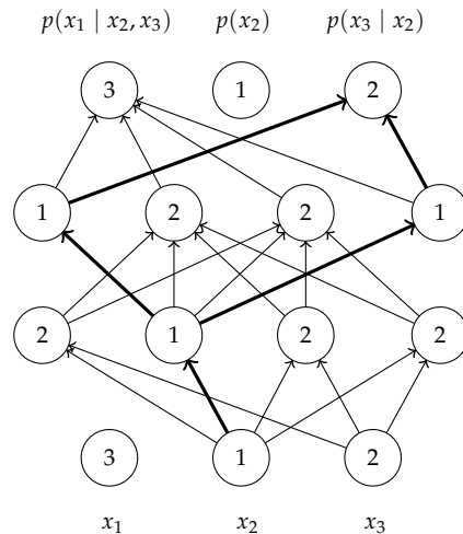
Figure 7.1. MADE masking with n = 3 .
