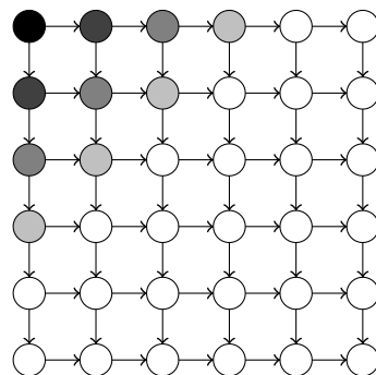
Figure 7.1. MADE masking with n = 3 .
