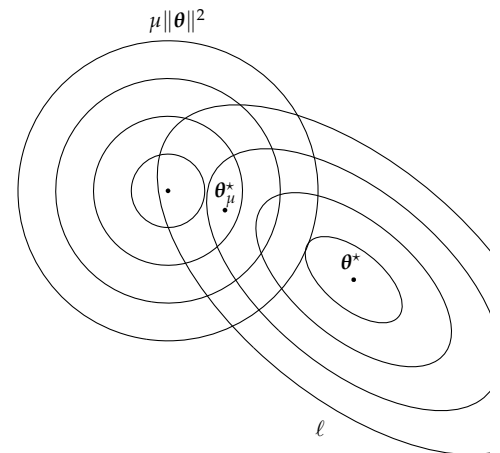
Figure 8.1. Loss landscape of an \ell_2 -regularized function.
