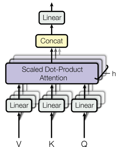
Figure 6.1. Multi-headed self-attention [Vaswani, 2017].
