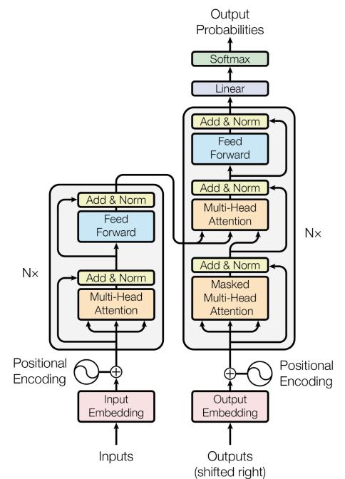
Figure 6.3. Architecture of the transformer [Vaswani, 2017]. The left side is called the encoder, which encodes the input sentence. The right side is called the decoder, which uses cross-attention to incorporate information from the source sequence in the prediction of the target sequence. The model works in an autoregressive manner, which means that the next token is predicted from the history until an end-of-sentence token is predicted.
