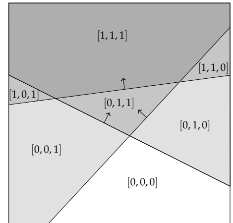
Figure 2.1. Connected regions, partitioned according to activation pattern. Each hyperplane represents a hidden unit. This shows an MLP with 2-dimensional input and 3-dimensional hidden layer.
